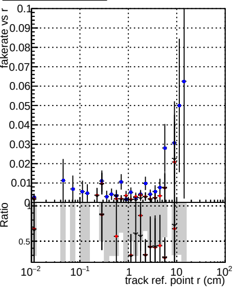
Fake rate vs vertpos —●— DOMstep3 SoftQCD CKF —●— DOMstep3 SoftQCD default —●— DOMstep3 SoftQCD defaultNEW20
