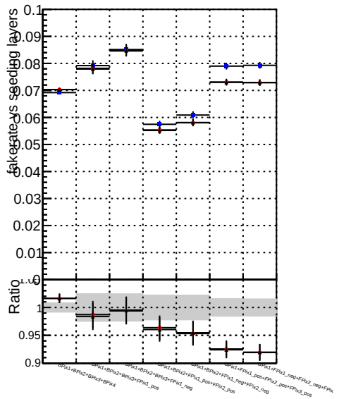
Fake rate vs. DOMstep3 SMS CKF DOMstep3 SMS CKF default DOMstep3 SMS CKF PixelLess
