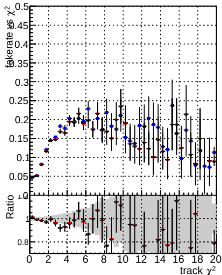
Fake rate vs. DOMstep3 SMS CKF DOMstep3 SMS CKF default DOMstep3 SMS CKF PixelLess
