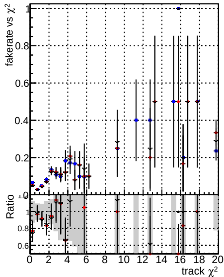
Fake rate vs. DOMstep3 SMS CKF DOMstep3 SMS default DOMstep3 SMS CKPixelLess
