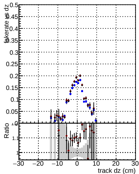
Fake rate vs dz — DOMstep3 SMS CKF — DOMstep3 SMS CKF default — DOMstep3 SMS CKF PixelLess
