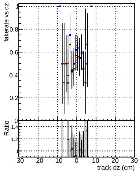
Fake rate vs dz Legend: DOMstep3 SMS CKF DOMstep3 SMS default DOMstep3 SMS CKFPixelLess
