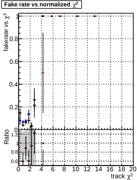
Fake rate vs. DOMstep3 SMS CKF DOMstep3 SMS default DOMstep3 SMS CKPixelLess
