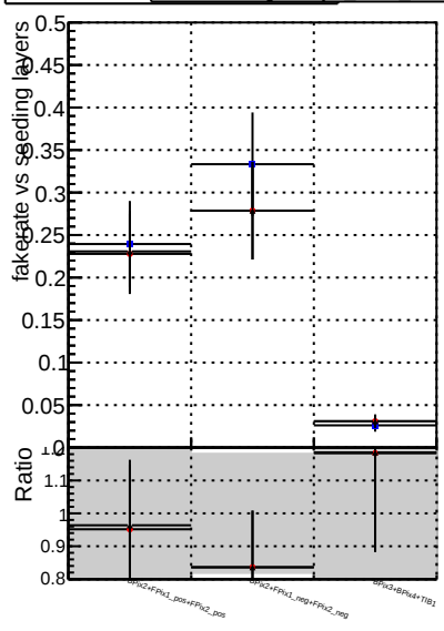
Fake rate vs. DOMstep3 SMS CKF DOMstep3 SMS default DOMstep3 SMS CKPixelLess
