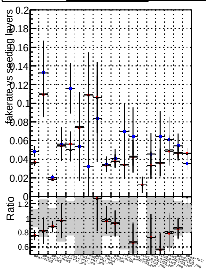
Fake rate vs. Legend: DOMstep3 SMS CKF (blue dots) DOMstep3 SMS default (red dots) DOMstep3 SMS CKPixelLess (black dots)
