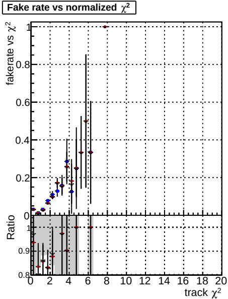
Fake rate vs. Legend: DOMstep3 SMS CKF (blue dots) DOMstep3 SMS default (red dots) DOMstep3 SMS CKPixelLess (black dots)
