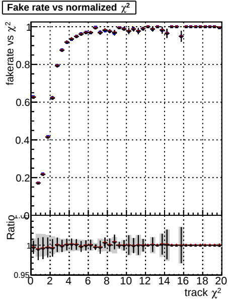
Fake rate vs. DOMstep3 SMS CKF DOMstep3 SMS default DOMstep3 SMS CKFPixelLess
