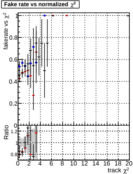
Fake rate vs. \chi^2 Legend: DOMstep3 SMS CKF DOMstep3 SMS default DOMstep3 SMS defaultNEWT
