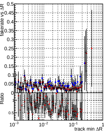
Fake rate vs \Delta R(\text{track, jet}) Legend: DQMstep3 SMS CKF (blue stars) DQMstep3 SMS default (red stars) DQMstep3 SMS defaultNEWT (black stars)
