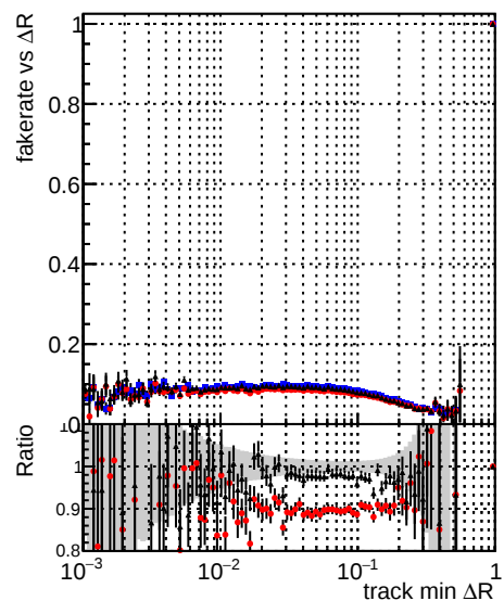
Legend for Fake rate vs \Delta R , Duplicates Rate vs \Delta R , and Pileup rate vs \Delta R : \blacksquare DQMstep3_QCD_CKF \bullet DQMstep3_QCD_default \times DQMstep3_QCD_ckfPixelLess
