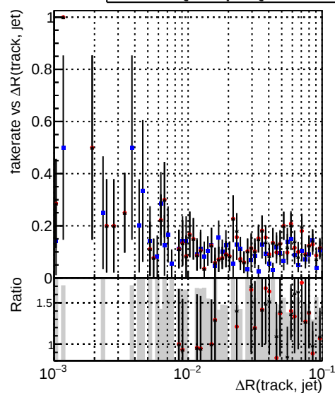
Legend for Fake rate vs \Delta R , Duplicates Rate vs \Delta R , and Pileup rate vs \Delta R : \blacksquare DQMstep3_QCD_CKF \bullet DQMstep3_QCD_default \times DQMstep3_QCD_ckfPixelLess
