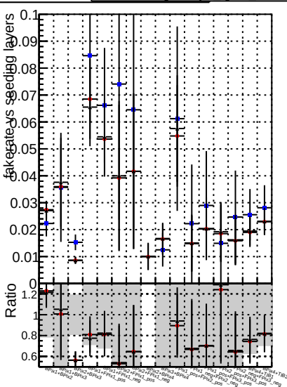
Fake rate vs. DOMstep3 OCB CKF DOMstep3 OCB default DOMstep3 OCB CKFPixelLess
