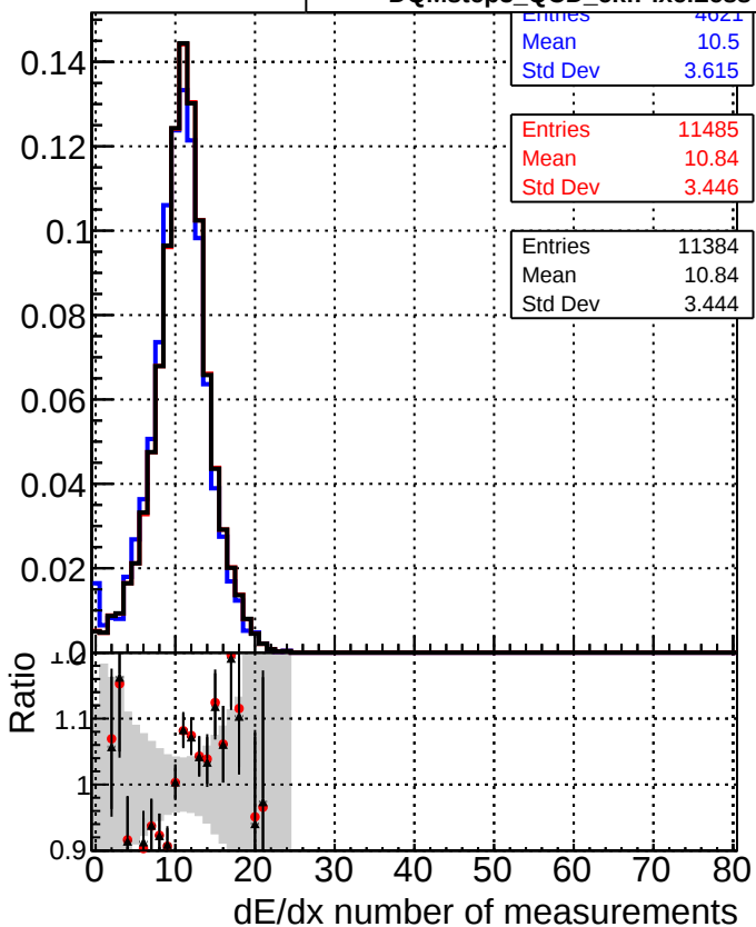
Legend for bottom row plots: DQMstep3_QCD_CKF (blue line with squares) DQMstep3_QCD_default (red line with circles) DQMstep3_QCD_ckfPixelLess (black line with crosses)
