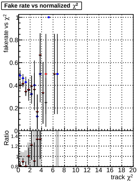
Fake rate vs. DOMstep3 OCB CKF OCB default OCB CKFPixelLess
