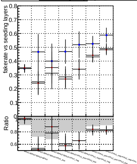
Fake rate vs. DOMstep3 OCB CKF OCB default OCB CKFPixelLess
