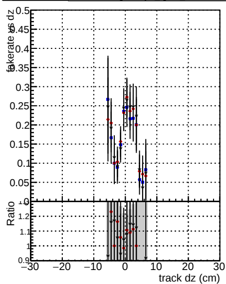
Fake rate vs dz Legend: DOMstep3 OCB CKF (black line with blue dots) DOMstep3 OCB default (red line with red dots) DOMstep3 OCB CRPixelLess (black line with black dots)
