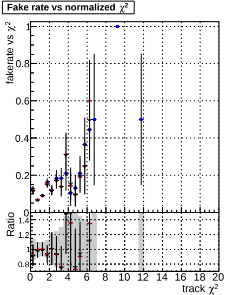
Fake rate vs. DOMstep3 OCB CKF DOMstep3 OCB default DOMstep3 OCB CKFPixelLess
