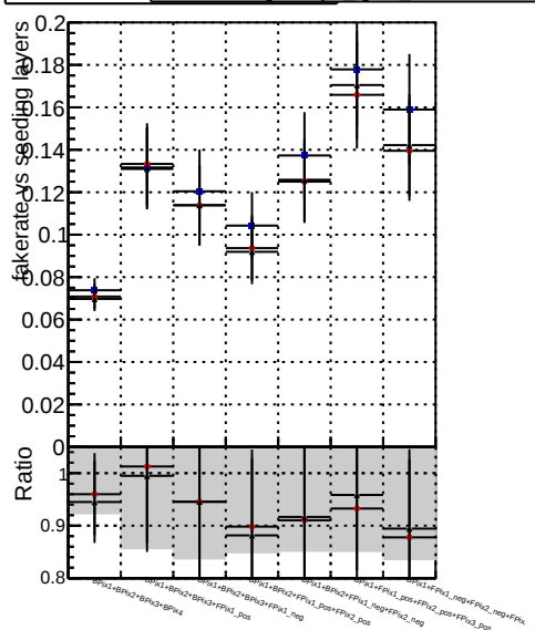
Fake rate vs. DOMstep3 OCB CKF DOMstep3 OCB default DOMstep3 OCB CKFPixelLess
