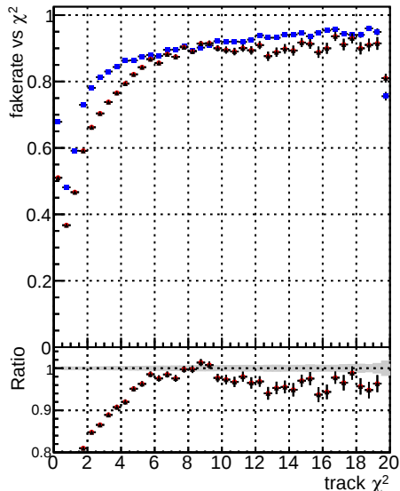
Fake rate vs. DOMstep3 OCB CKF DOMstep3 OCB default DOMstep3 OCB CKFPixelLess
