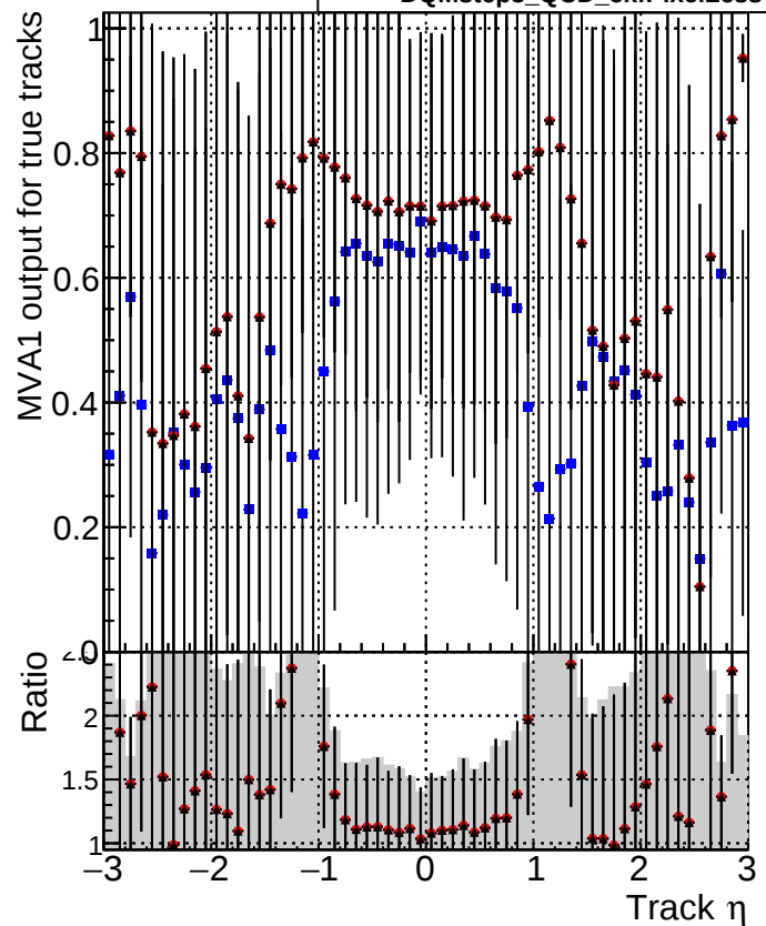
MVA1 of associated tracks (recoToSim) vs. track \eta Legend: ■ DQMstep3_QCD_CKF ● DQMstep3_QCD_default ▲ DQMstep3_QCD_ckfPixelLess
