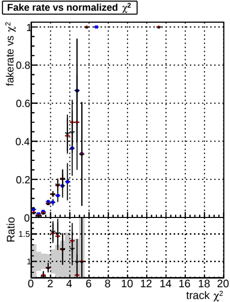
Fake rate vs. Legend: DOMstep3 OCB GKF DOMstep3 OCB default DOMstep3 OCB CRPixelLess
