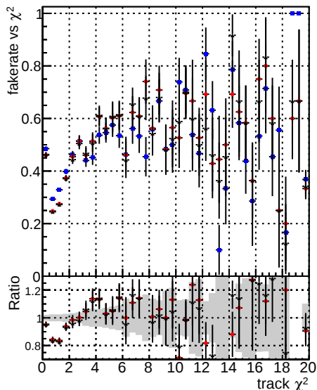
Fake rate vs. Legend: DOMstep3 OCB GKF (blue diamonds) DOMstep3 OCB default (red crosses) DOMstep3 OCB CRPixelLess (black crosses)
