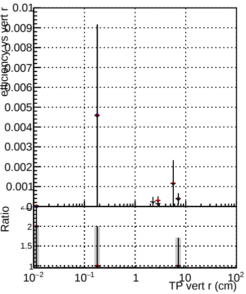
Efficiency vs. TP vert r (cm) Legend: DQMstep3_QCD_CKF (blue line with dots) DQMstep3_QCD_default (red line with dots) DQMstep3_QCD_defaultNEWT (black line with dots)
