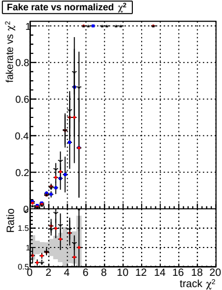
Fake rate vs. Legend: DOMstep3 OCB CKF (blue stars) DOMstep3 OCB default (red stars) DOMstep3 OCB defaultNEWT (black stars)
