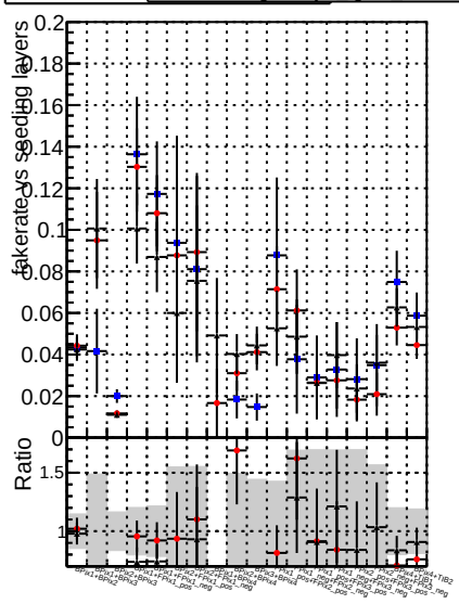
Fake rate vs. Legend: DOMstep3 OCB CKF (blue stars) DOMstep3 OCB default (red stars) DOMstep3 OCB defaultNEWT (black stars)
