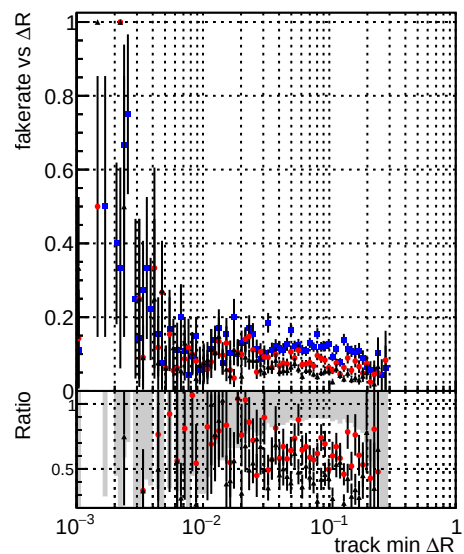
Legend for Fake rate vs \Delta R , Duplicates Rate vs \Delta R , and Pileup rate vs \Delta R : DQMstep3_QCD_CKF (blue circles) DQMstep3_QCD_default (red circles) DQMstep3_QCD_defaultNEWT (black circles)
