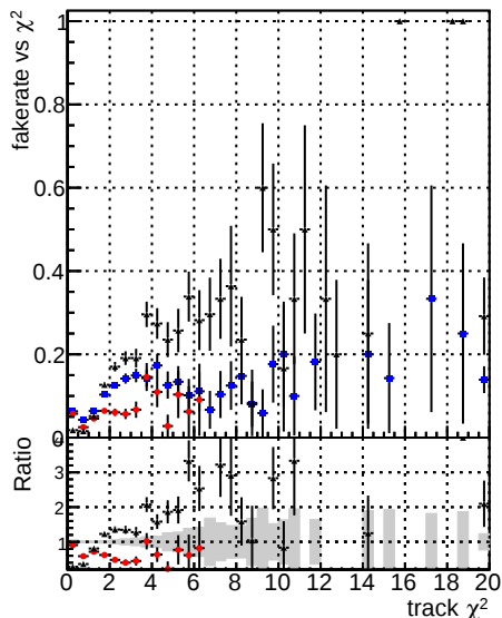
Fake rate vs. DOMstep3 OCB CKF OCB default NEWT Blue diamond Black cross Red cross Grey cross
