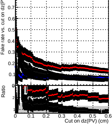
Fake rate vs. cut on dz(PV)
