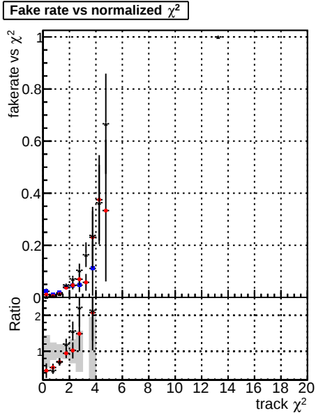
Fake rate vs. Legend: DOMstep3 OCB CKF (blue), DOMstep3 OCB default (red), DOMstep3 OCB defaultNEWT (black)
