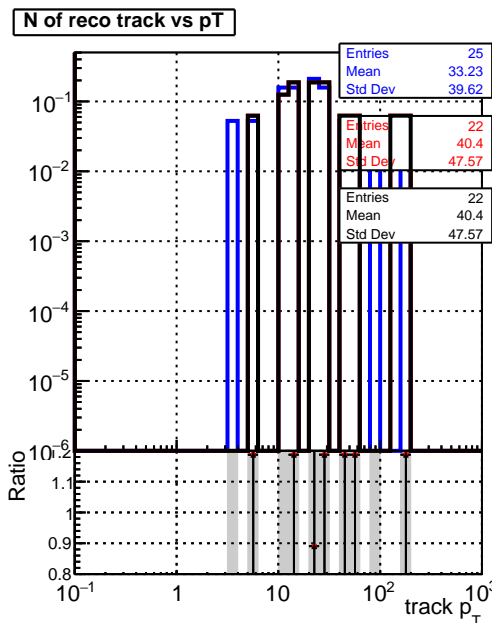
N of reco track vs pT
