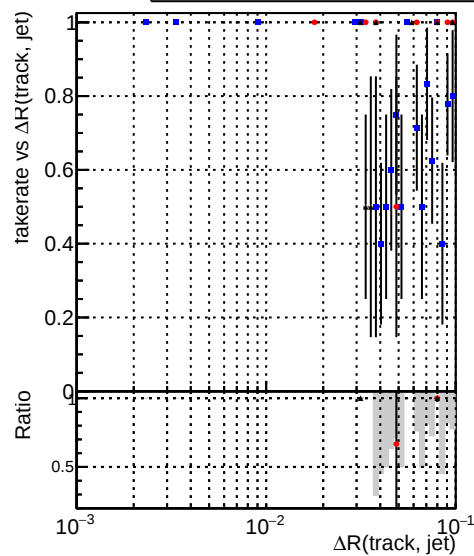
Legend for Fake rate vs \Delta R , Duplicates Rate vs \Delta R , and Pileup rate vs \Delta R : DQMstep3_QCD_CKF (Blue diamonds) DQMstep3_QCD_default (Red stars) DQMstep3_QCD_defaultNEWT (Black crosses)
