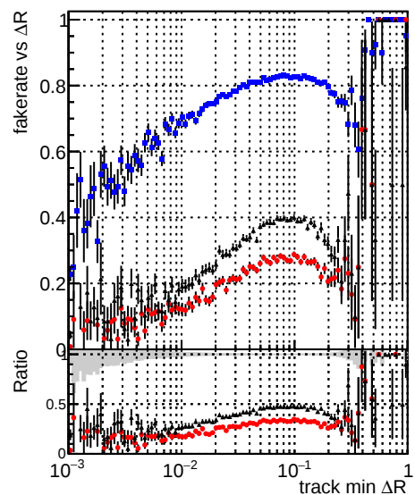
Legend for Fake rate vs \Delta R , Duplicates Rate vs \Delta R , and Pileup rate vs \Delta R : DQMstep3_QCD_CKF (Blue diamonds) DQMstep3_QCD_default (Red stars) DQMstep3_QCD_defaultNEWT (Black crosses)
