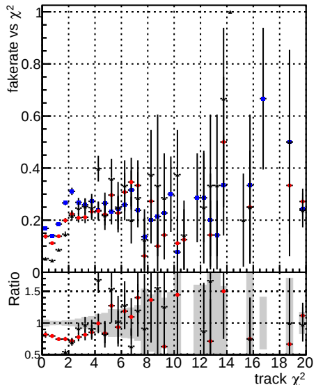
Fake rate vs. DOMstep3 OCB CKF DOMstep3 OCB default NEWT
