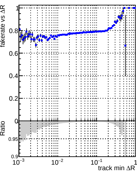
Fake rate vs \Delta R(\text{track}, \text{jet}) DQMstep3_QCD_defaultCHECK
