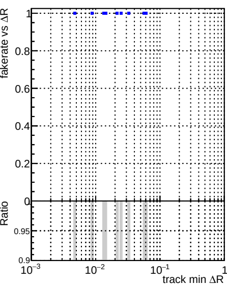
Fake rate vs \Delta R(\text{track, jet}) DQMstep3_QCD_defaultCHECK
