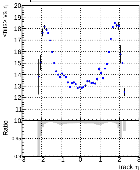
mean hits vs \eta DQMstep3_QCD_defaultCHECK
