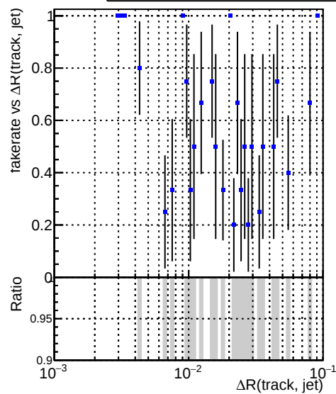
Fake rate vs \Delta R(\text{track, jet}) DQMstep3_QCD_defaultCHECK
