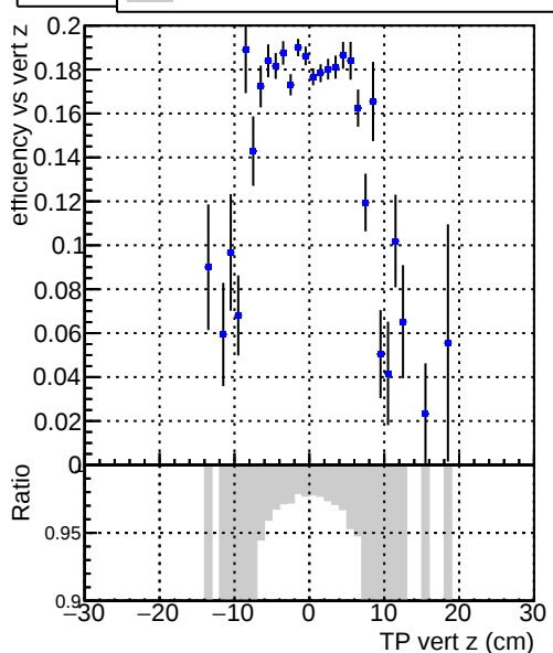
Efficiency vs. DQMstep3_QCD_defaultCHECK
