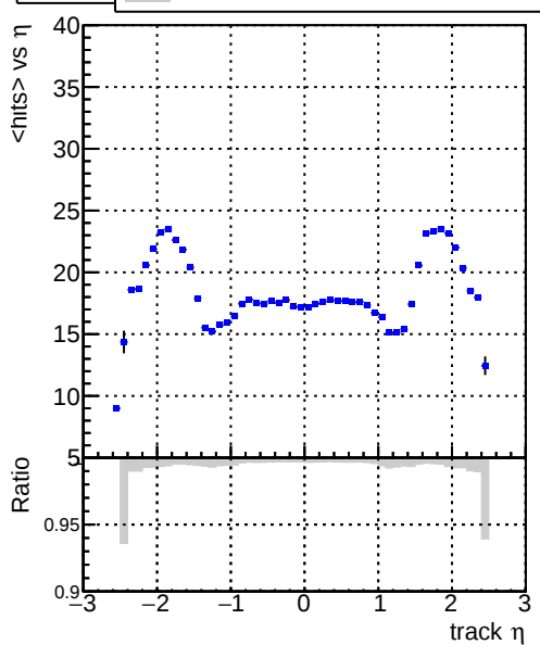
mean hits vs \eta DQMstep3_QCD_defaultCHECK
