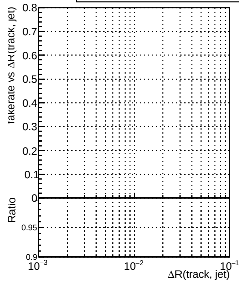
Fake rate vs \Delta R(\text{track}, \text{jet}) DQMStep3_QCD_defaultCHECK
