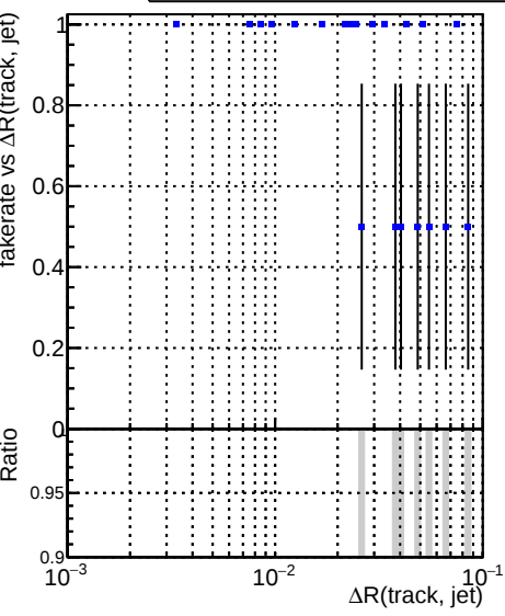
Fake rate vs \Delta R(\text{track, jet}) DQMstep3_QCD_defaultCHECK
