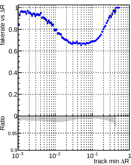
Fake rate vs \Delta R (track, jet) DQMStep3_QCD_defaultCHECK
