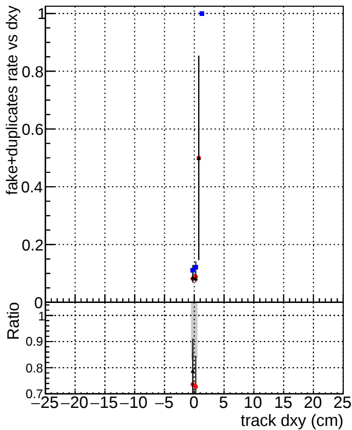
Legend for the plots: DQMstep3_DisplacedSUSY_CKF (Blue squares) DQMstep3_DisplacedSUSY_default (Red circles) DQMstep3_DisplacedSUSY_ckfPixelLess (Black triangles)
