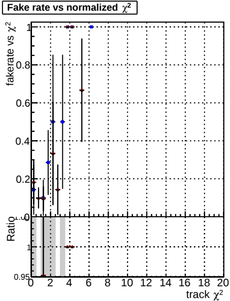
Fake rate vs. DOMstep3 DisplacedSUSY CKF DOMstep3 DisplacedSUSY default DOMstep3 DisplacedSUSY CKFPixelLess
