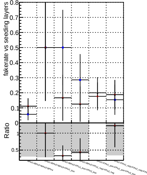
Fake rate vs. DOMstep3 DisplacedSUSY CKF DOMstep3 DisplacedSUSY default DOMstep3 DisplacedSUSY CKFPixelLess
