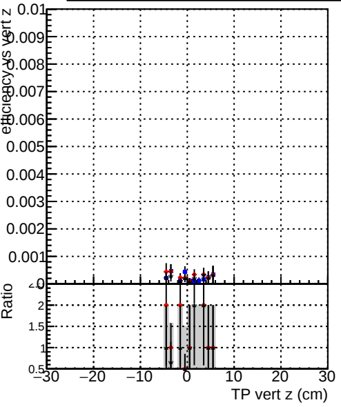
Efficiency vs. TP vert z Legend: DQMstep3_DisplacedSUSY_CKF (Blue line with markers) DQMstep3_DisplacedSUSY_default (Red line with markers) DQMstep3_DisplacedSUSY_defaultNEWT (Black line with markers)
