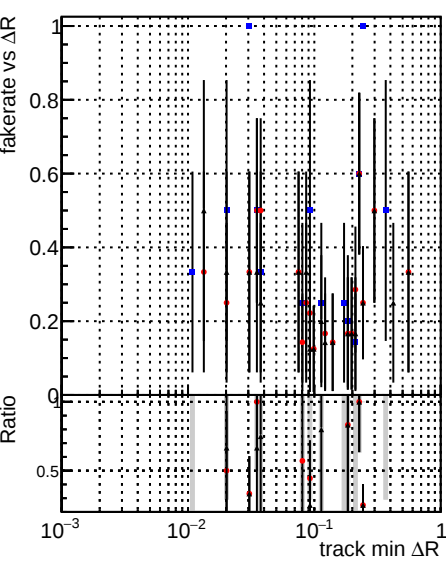
Legend: DQMstep3_DisplacedSUSY_CKf (blue dots), DQMstep3_DisplacedSUSY_default (red dots), DQMstep3_DisplacedSUSY_NEWT (black dots)
