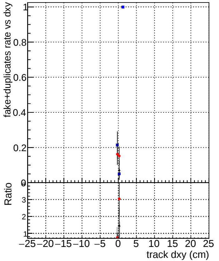
Legend for the bottom plot: DQMstep3_DisplacedSUSY_CKF (Blue square) DQMstep3_DisplacedSUSY_default (Red circle) DQMstep3_DisplacedSUSY_defaultNEWT (Black triangle)
