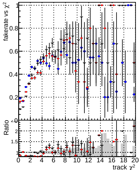
Fake rate vs. \chi^2 Legend: DOMstep3 DisplacedSUSY CKF (blue diamonds) DOMstep3 DisplacedSUSY default (red stars) DOMstep3 DisplacedSUSY default+NEWT (black crosses)
