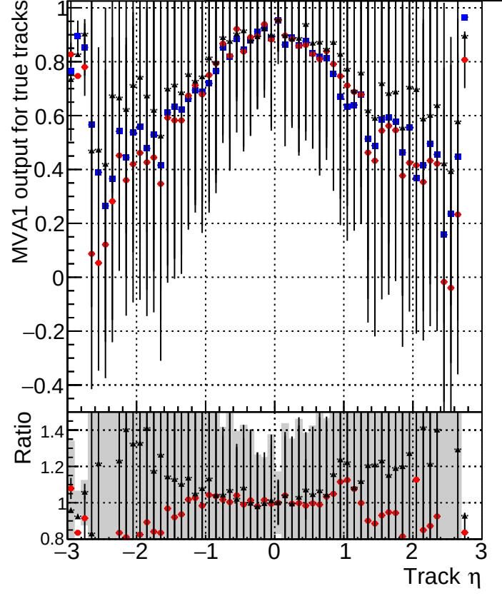
MVA1 of associated tracks (recoToSim) vs. track \eta Legend: ■ DQMstep3_DisplacedSUSY_CKF ● DQMstep3_DisplacedSUSY_default ★ DQMstep3_DisplacedSUSY_defaultNEWT
