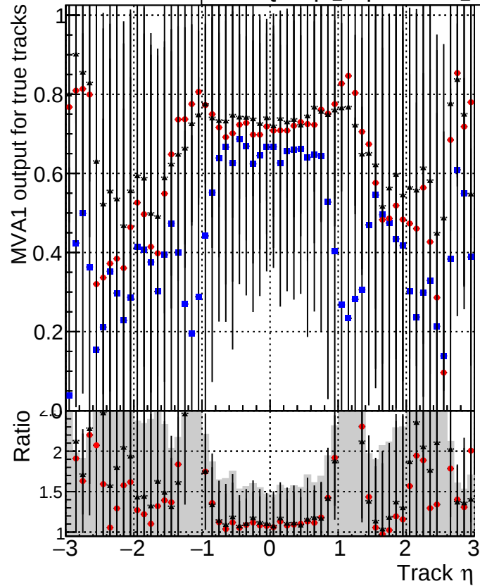
MVA1 of associated tracks (recoToSim) vs. track \eta Legend: ■ DQMstep3_DisplacedSUSY_CKF ◆ DQMstep3_DisplacedSUSY_default ★ DQMstep3_DisplacedSUSY_defaultNEWT
