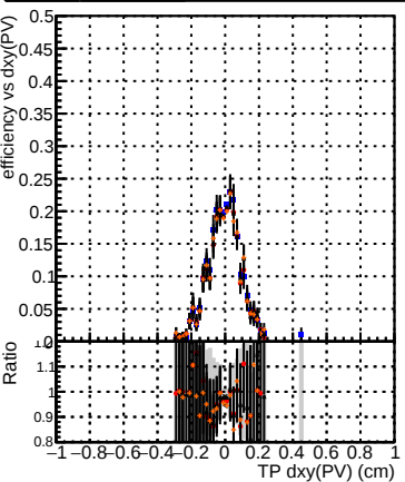
Efficiency vs Dxy(PV) plot. The x-axis is TP dxy(PV) (cm) and the y-axis is efficiency vs dxy(PV). The legend indicates the data sources: DQM_TT_mkFit-DQM_original, /data2/legianni/standalone-May24/CMSSW_13_2_X_2023-06-05-1100/src/DQM_TT_mkFit-DQM_mod_updatedmod-127, DQM_TT_mkFit-DQM_update-mod127, and DQM_TT_mkFit-DQM_127-updatemod127.
