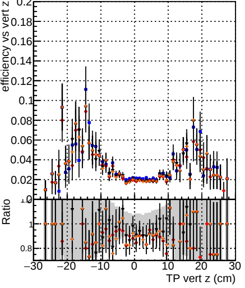
Efficiency vs vertpos Legend: —•— DQM TT mkFit-DQM original —•— /data2/legianni/standalone-May24/CMSSW_13_2_X_2023-06-05-1100/src/DQM TT_mkFit-DQM_mod_updatedmod-127 —•— DQM TT_mkFit-DQM_update-mod127 —•— DQM TT_mkFit-DQM_127-updatemod127
