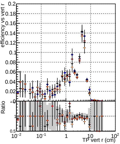
Efficiency vs vertpos Legend: —•— DQM TT mkFit-DQM original —•— /data2/legianni/standalone-May24/CMSSW_13_2_X_2023-06-05-1100/src/DQM TT_mkFit-DQM_mod_updatedmod-127 —•— DQM TT_mkFit-DQM_update-mod127 —•— DQM TT_mkFit-DQM_127-updatemod127
