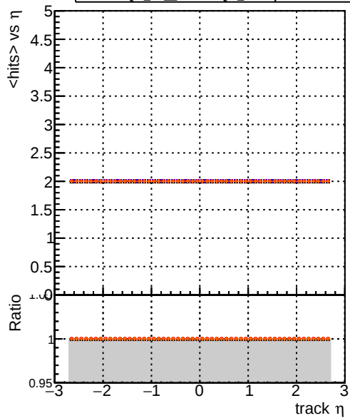
mean hits vs \eta Legend: Blue line: DQM TT mkFit-DQM original Red line: /data2/legianni/standalone-May24/CMSSW_13_2_X_2023-06-05-1100/src/DQM TT_mkFit-DQM_mod_updatedmod-127 Black line: DQM TT mkFit-DQM_update-mod127 Orange line: DQM TT mkFit-DQM_127-updatemod127
