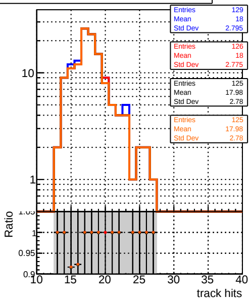
DQM TT_mkFit-DQM original /data2/legianni/standalone-May24/CMSSW_13_2_X_2023-06-05-1100/src/DQM TT_mkFit-DQM_mod_updatedmod127 DQM TT_mkFit-DQM_127-updatemod127
